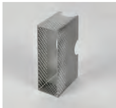
55 WALL BOX (1817) h.116mm w.52mm d.100mm h.4.56" w.2.04" d.3.93"
